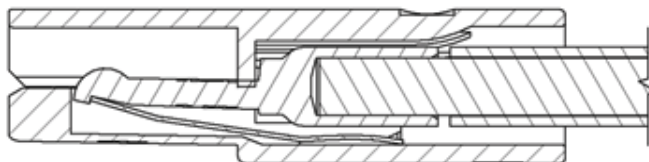
Contatto installato nella custodia Installed contact into housing
